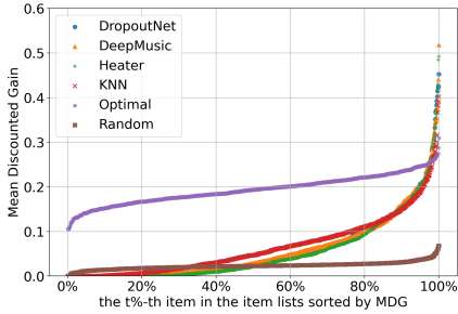
Figure 2: For ML1M and each model, sort items by MDG in ascending order and plot their corresponding MDG.
