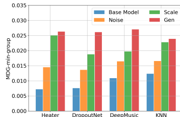
Figure 7: Investigate group-level fairness on ML1M.
